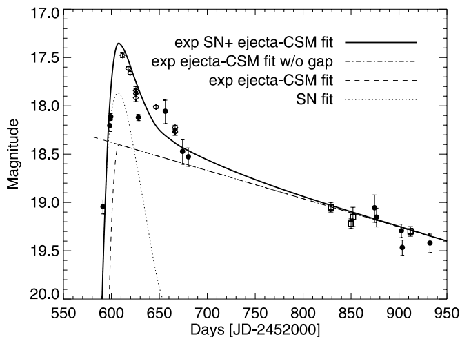
FIG. 5.—Observed photometry compared with the SN + exponential ejecta-CSM model described in § 6. [See the electronic edition of the Journal for a color version of this figure.]
