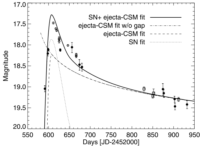
FIG. 3.—Observed photometry compared with the SN + power law ejecta-CSM model described in § 5. [See the electronic edition of the Journal for a color version of this figure.]
