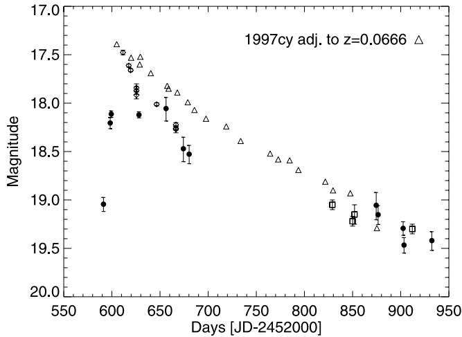
FIG. 4.—NEAT unfiltered and Hamuy V -band observations of SN 2002ic compared to the K -corrected V -band observations of SN 1997cy from Germany et al. (2000). No date of maximum or magnitude uncertainties are available for SN 1997cy. Here the maximum observed magnitude for SN 1997cy has been adjusted to the redshift of SN 2002ic, z = 0.0666 (Hamuy et al. 2003b), and the date of the first light curve point of SN 1997cy has been set to the date of maximum for SN 2002ic from our V -band fit. [See the electronic edition of the Journal for a color version of this figure.]
