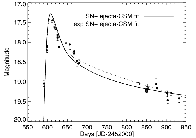
FIG. 6.—Comparison of fits with power-law (solid line) and exponential (dotted line) SN ejecta density profiles. [See the electronic edition of the Journal for a color version of this figure.]
