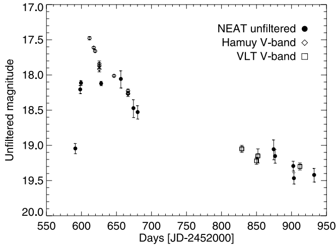
FIG. 1.—Unfiltered optical light curve of SN 2002ic as observed by NEAT with the Palomar 1.2 m and Haleakala 1.2 m telescopes (see Table 1). Magnitudes have been calibrated against the USNO-A1.0 POSS-E stars in the surrounding field. No color correction has been applied. Also shown are the observed V -band magnitudes from Hamuy et al. (2003b) and V -band magnitudes from the spectrophotometry of Wang et al. (2004). [See the electronic edition of the Journal for a color version of this figure.]
