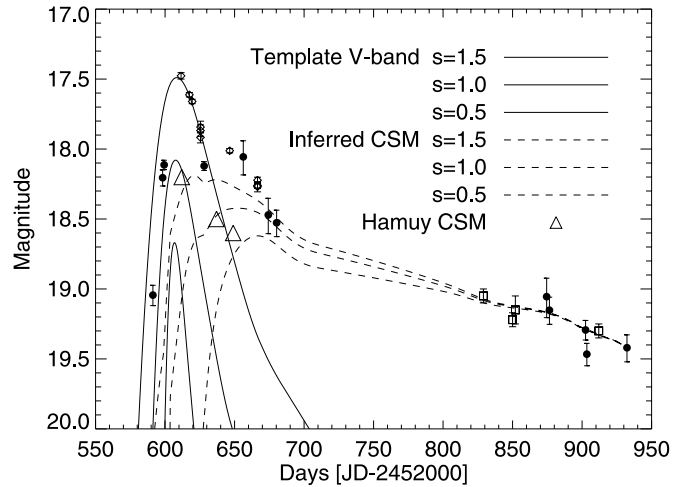
FIG. 2.—Template SN Ia V -band light curve (solid lines; stretch decreases from top to bottom line) shown for comparison with the photometric observations at several stretch values s , where the magnitude-stretch relation \Delta m = 1.18(1 - s) has been applied. The difference between the observed photometry points and the template fit has been smoothed over a 50 day window (dashed lines). Note that an assumption of no CSM contribution in the first 15 days after maximum light (i.e., s = 1.5 ) is in conflict with the spectroscopic measurements of Hamuy et al. (2003b) (open triangles; no error bars available). [See the electronic edition of the Journal for a color version of this figure.]
